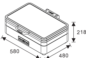
W20-1102T Induction Chafer W07-1101B Electrical Base Open Lid Height: 655mm
