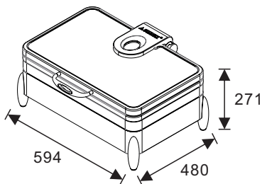
W07-1102T Induction Chafers W07-1104B Multi-Functional Base Open Lid Height: 687mm
